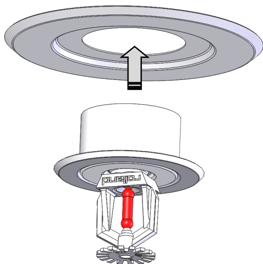
Assembly with two pieces escucheon
